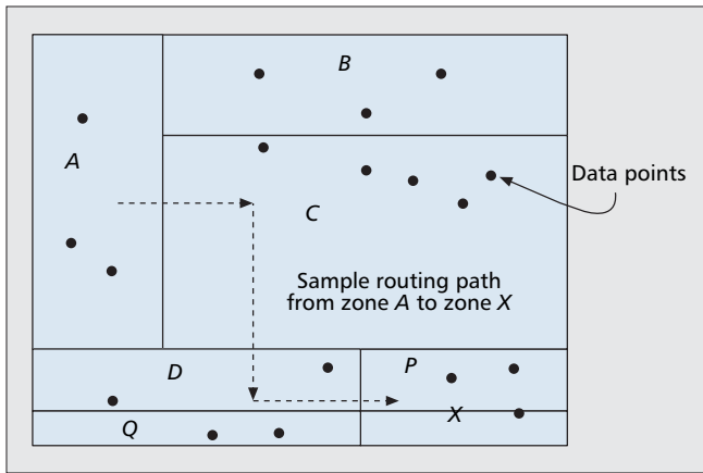
Figure 13. Example routing in a 2-dimensional CAN space that utilizes k - d tree index to organize d -dimensional data. Peer X 's coordinate neighbor set = \{D, P, Q\} ; peer A 's coordinate neighbor set = \{B, C, D\} ; peer C 's coordinate neighbor set = \{A, B, D, P\} , peer D 's coordinate neighbor set = \{A, C, P, X, Q\} .
