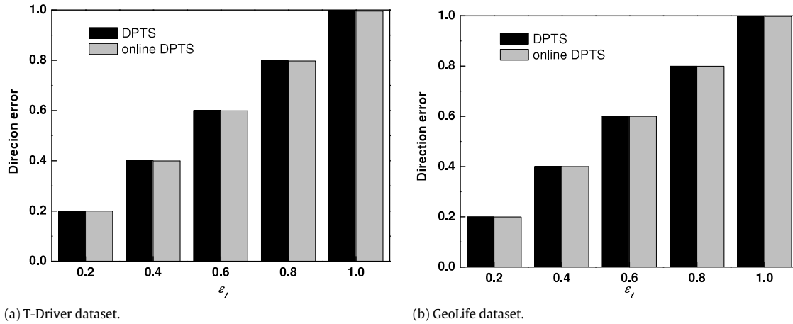
Fig. 6. The comparison of direction error with DPTS.
