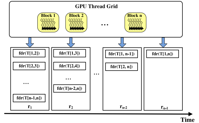
Fig. 4. The parallel scheme for constructing graph.
