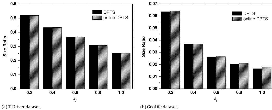
Fig. 8. The compression rate of online DPTS.
