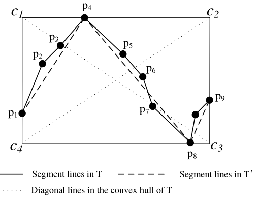
Fig. 2. Example of bounding L_{\max} .
