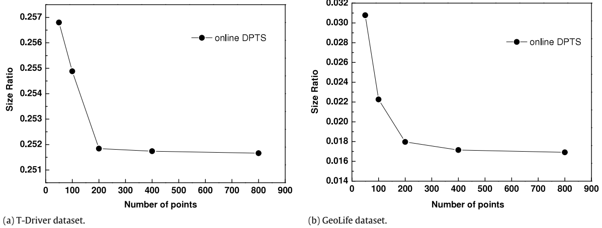
Fig. 7. The effect of segment size on online DPTS.
