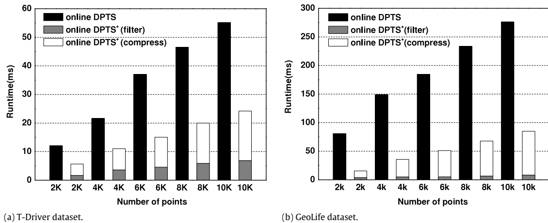
Fig. 13. The runtime of online DPTS + .
