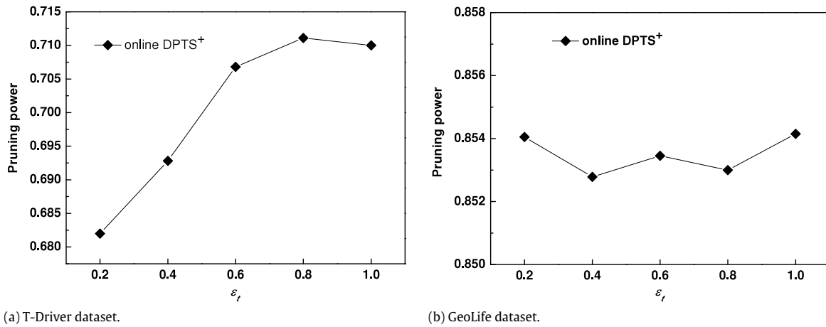
Fig. 12. The pruning power of online DPTS + .
