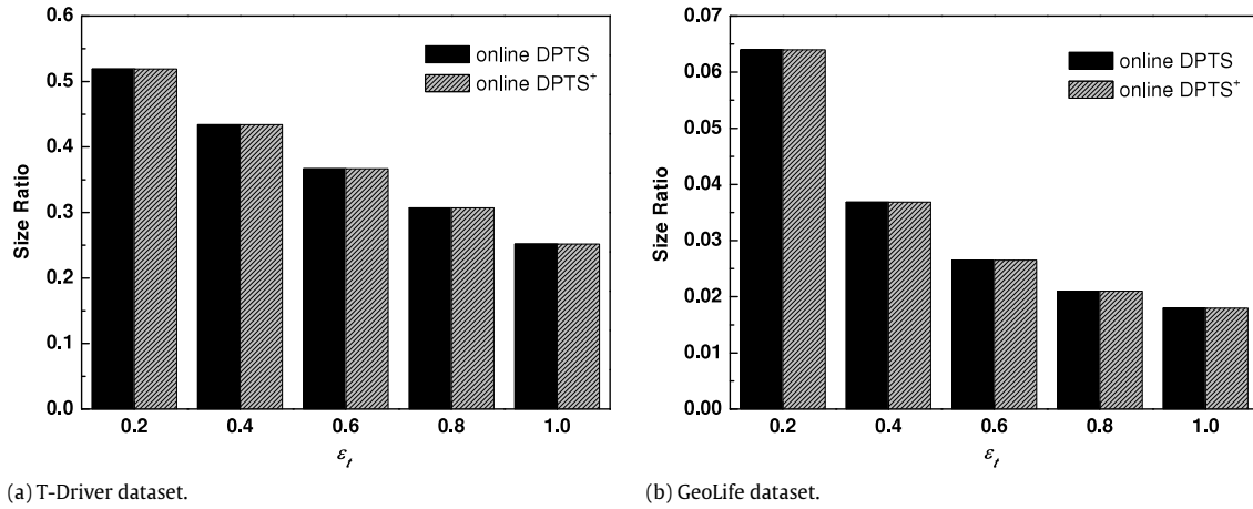
Fig. 11. The compression rate of online DPTS + .
