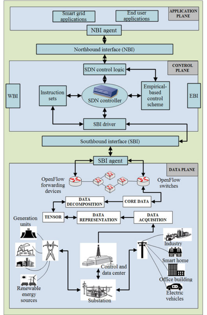
Fig. 4. Tensor-based SDN model.
