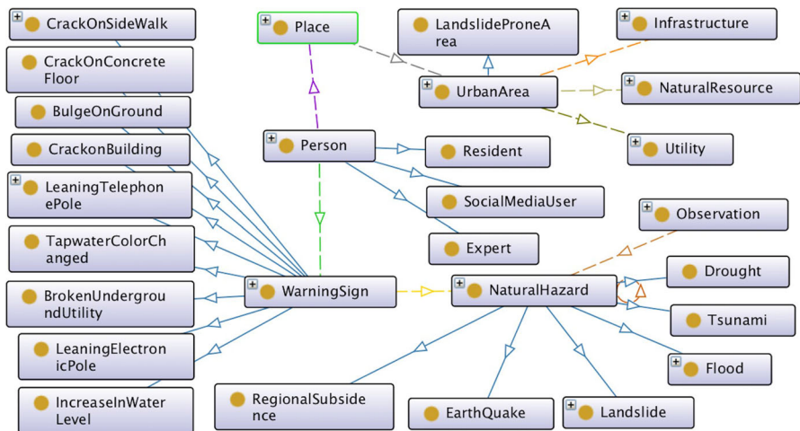
Fig. 3 Common Ontology
