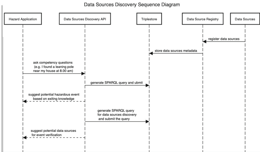
Fig. 6 Data Sources Discovery Sequence Diagram
