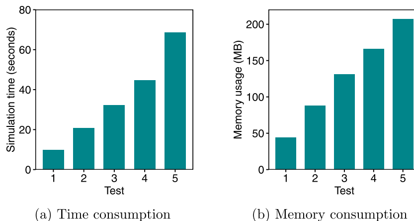
Fig. 11. Simulation complexity.
